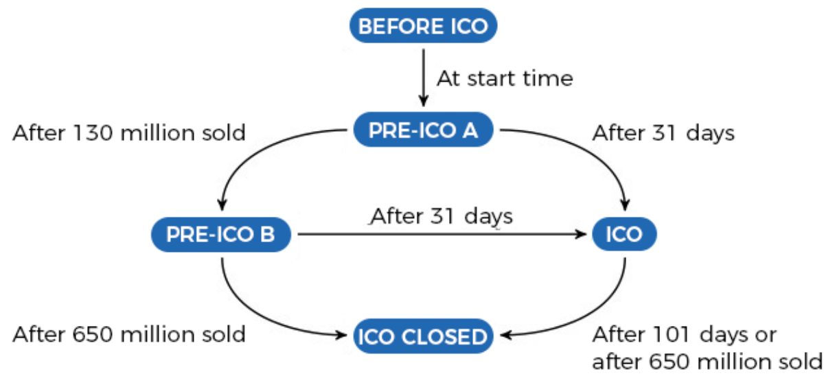
Figure 2: State Transitions for the Crowdsale.
